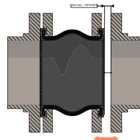
Figure 4: Axial Misalignment
