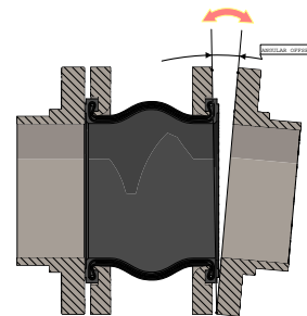
Figure 6: Angular Misalignment
