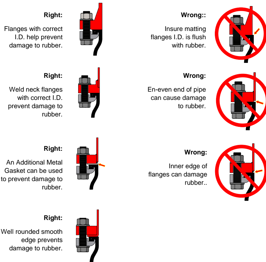
Figure 16: Flange Preparation
