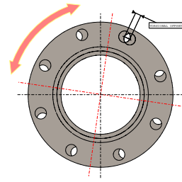
Figure 7: Torsional Misalignment
