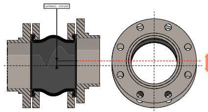
Figure 5: Lateral Misalignment
