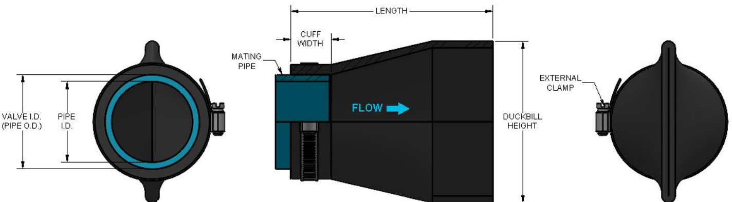
Detail of the ProFlex™ Slip-on Rubber Check Valve; Style 730M
